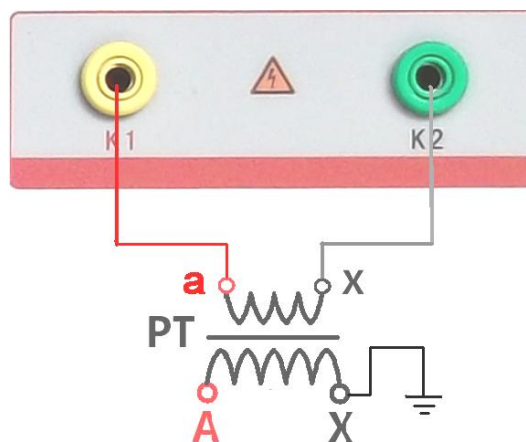
Figure 3(PT Excitation Connection Diagram)
