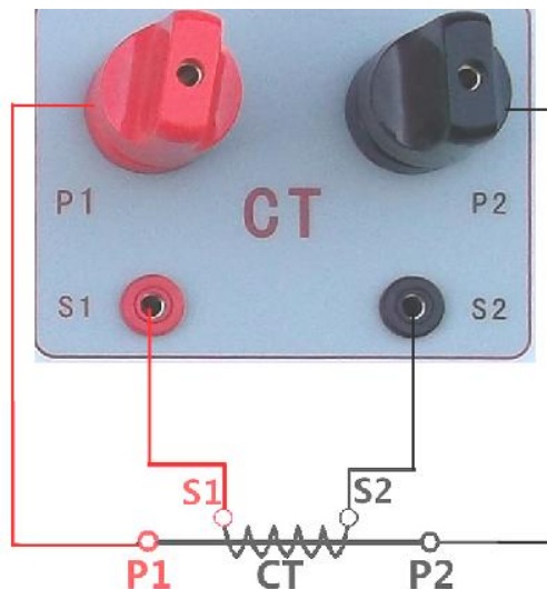
Figure 5 (CT Connection Diagram for Transformation Ratio, Polarity)
