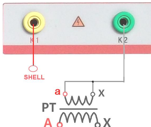
Figure 8 (PT Connection Diagram for Withstand Test of Alternating Current)
