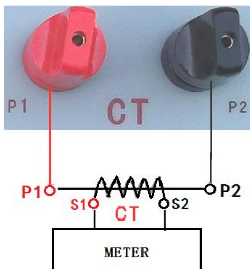
Figure 4 (CT Current Output Connection Diagram)
