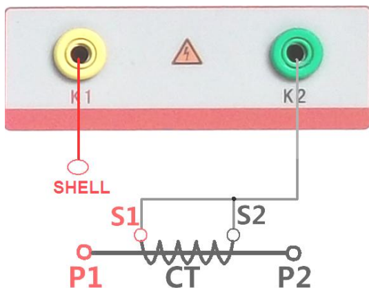
Figure 7 (CT Connection Diagram for Withstand Test of Alternating Current)
